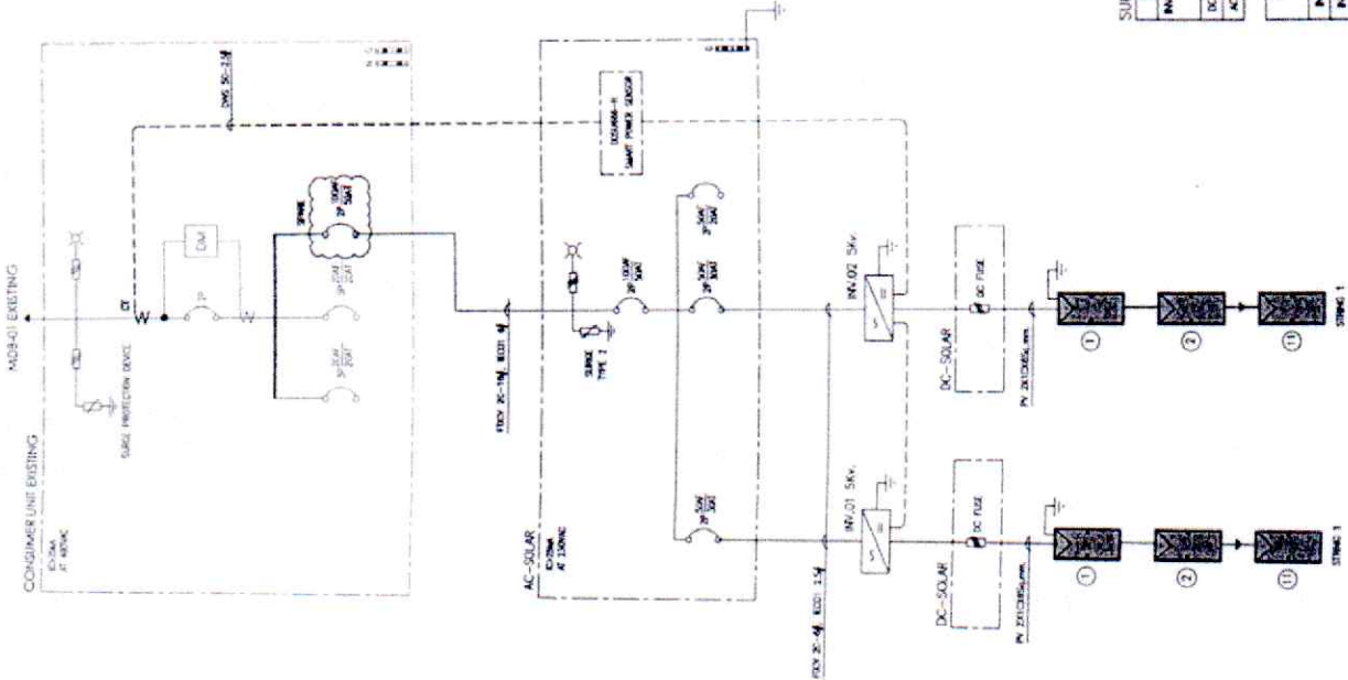
SINGLE LINE DIAGRAM INVERTER SCALE: NONE
